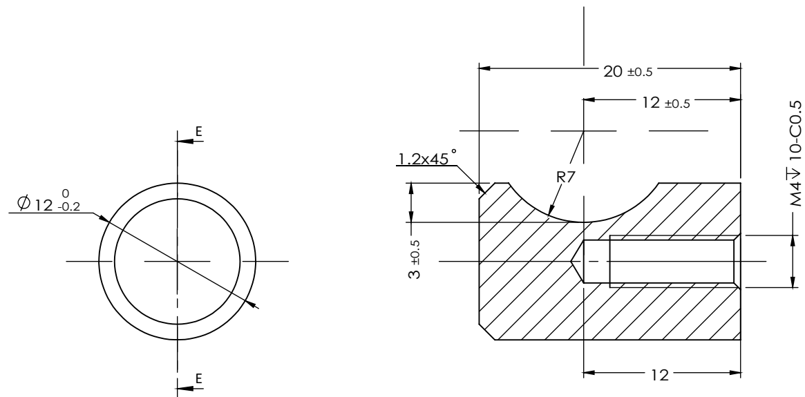
Section E-E
